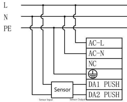
Wiring diagram of corridor dimming
